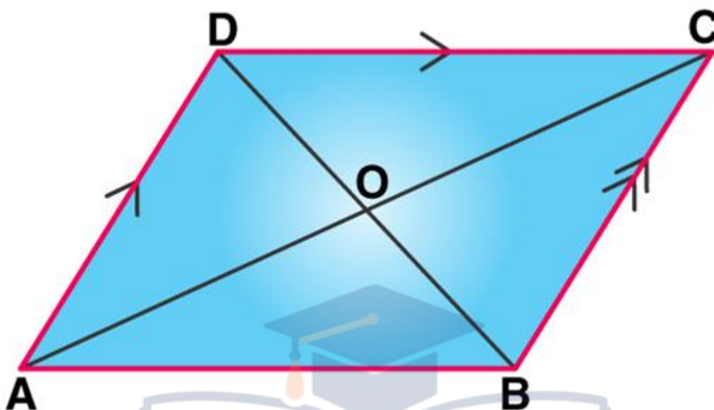
Parallelogram
